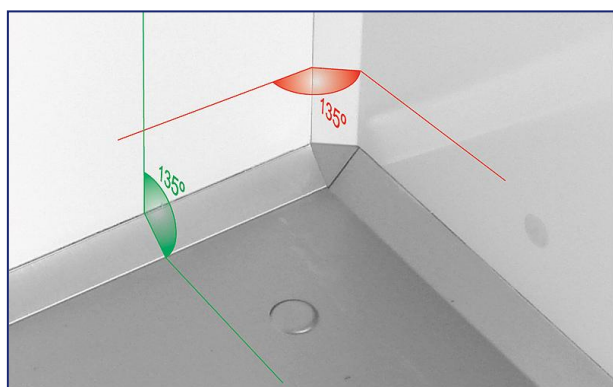
Preformed sanitary corners (135° wide angle)
