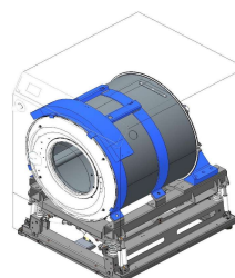
MECCANICA MECHANICS
