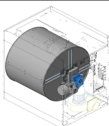
TRASMISSIONE TRANSMISSION
