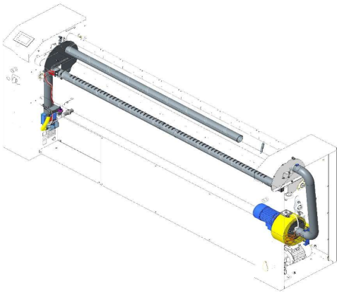
RISCALDAMENTO GAS GAS HEATING
