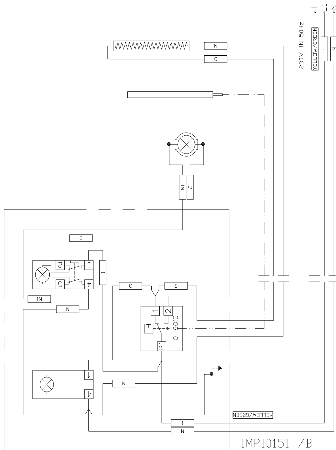
Fig. 9.1 Electrical diagram at 230Vac single phase
