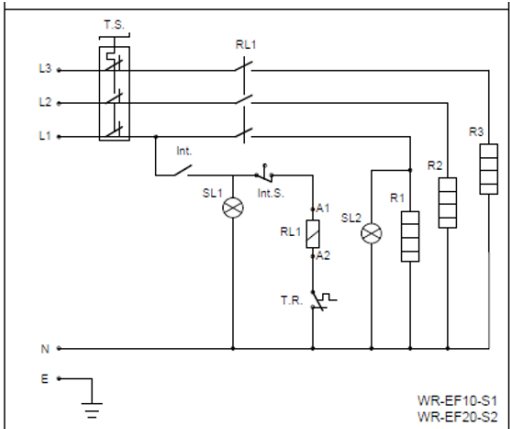
Fig.2 (sch3mas 3lectriques)
