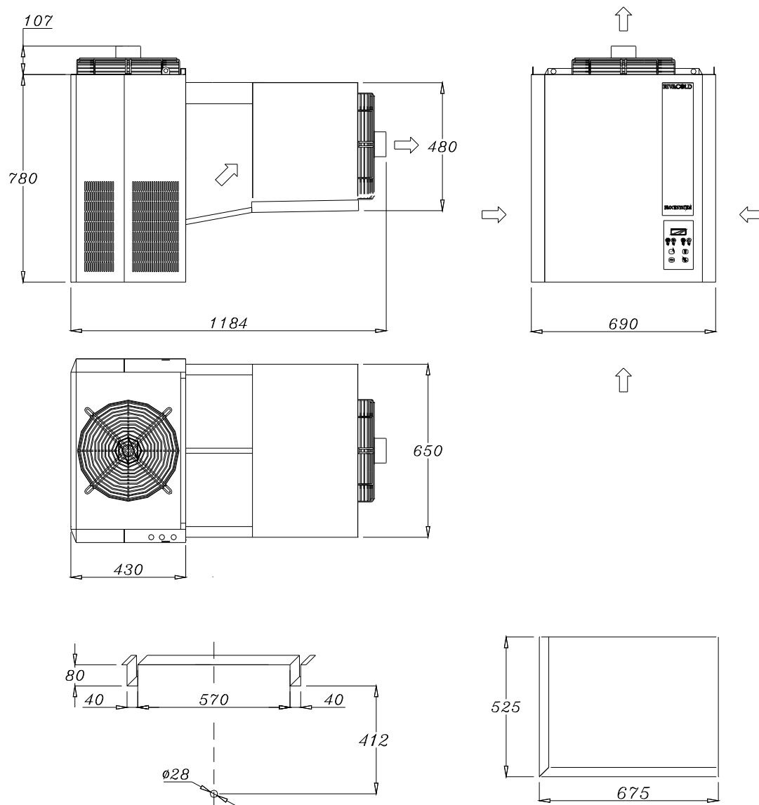
Drawing. 10 (1x350)
