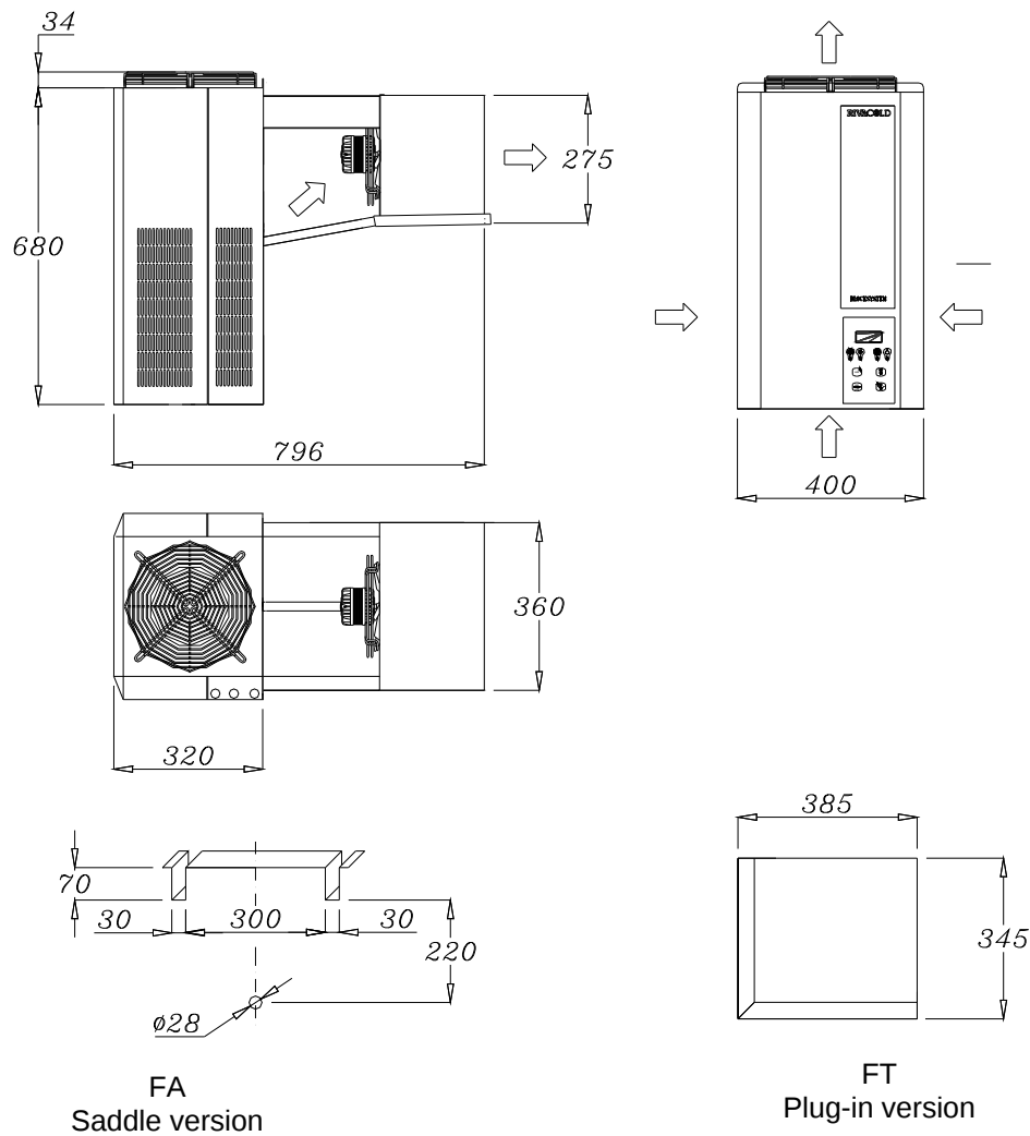
Drawing. 8 (1X250)
