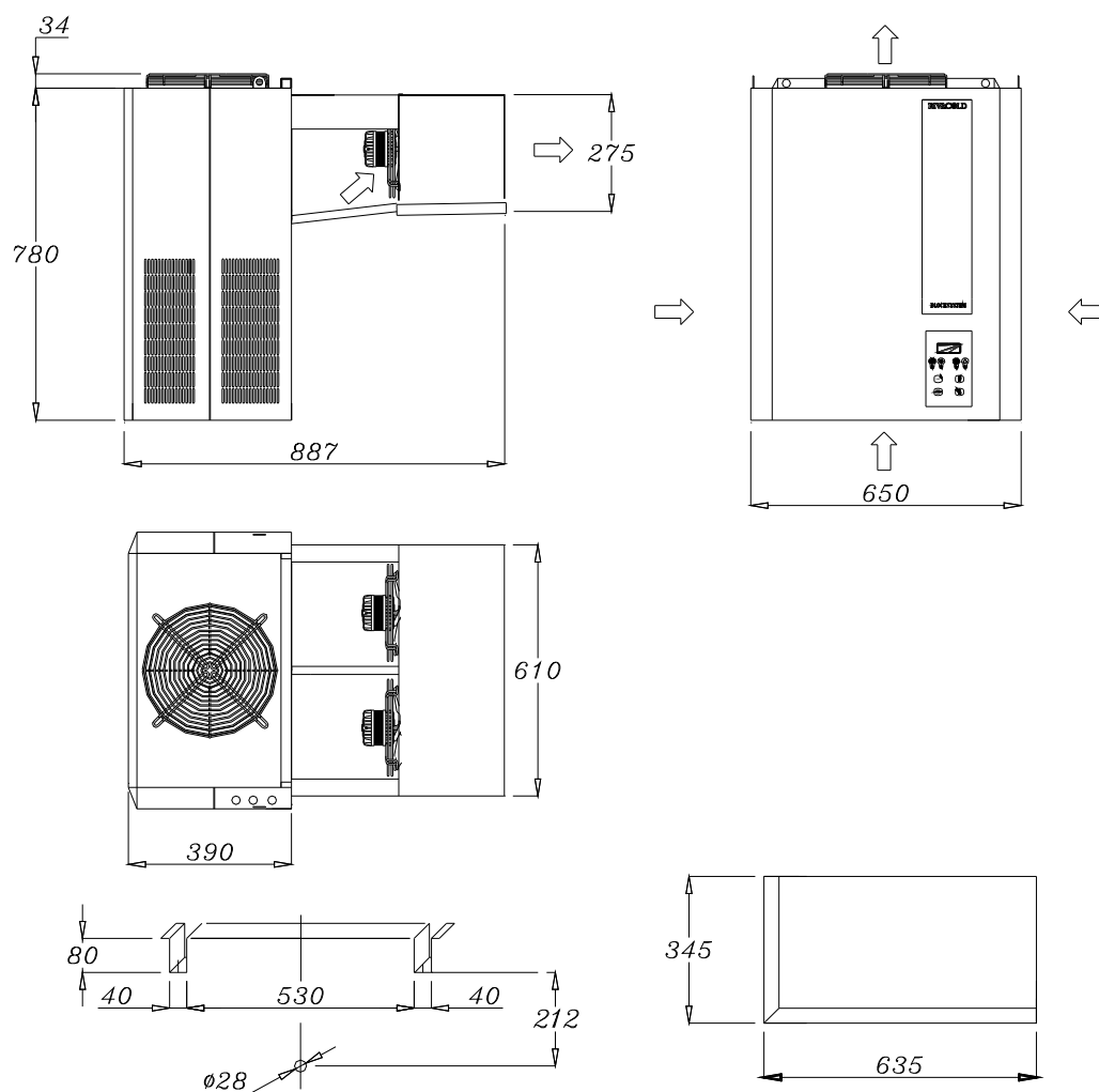
Drawing. 9 (1X300)
